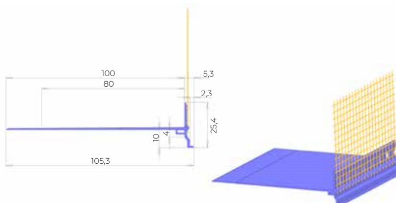
PVC Terminal with mesh
