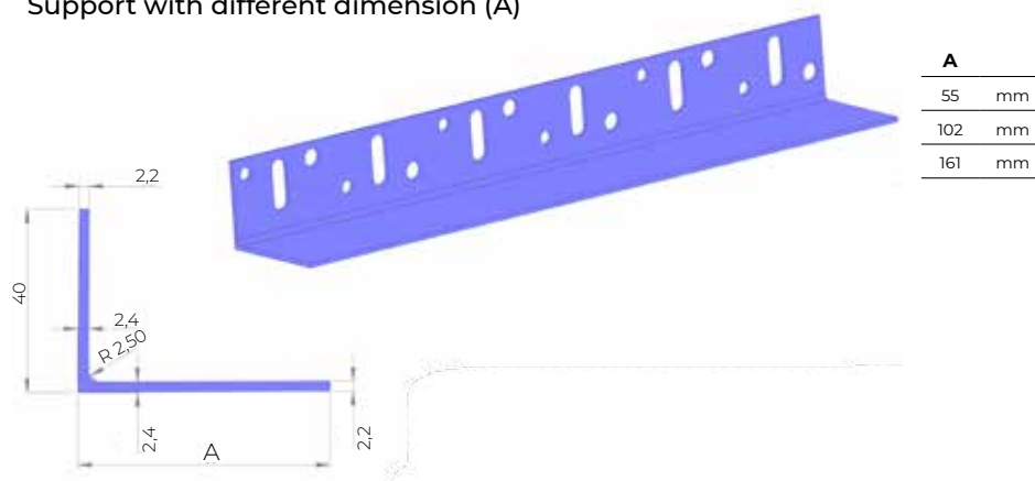
Support with different dimension (A)
