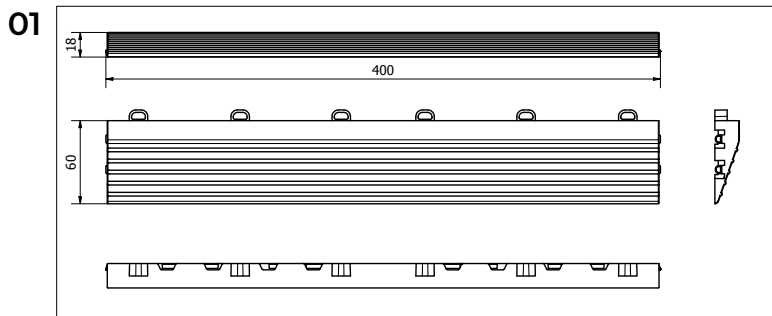
01 Ramp with "female" hooking
